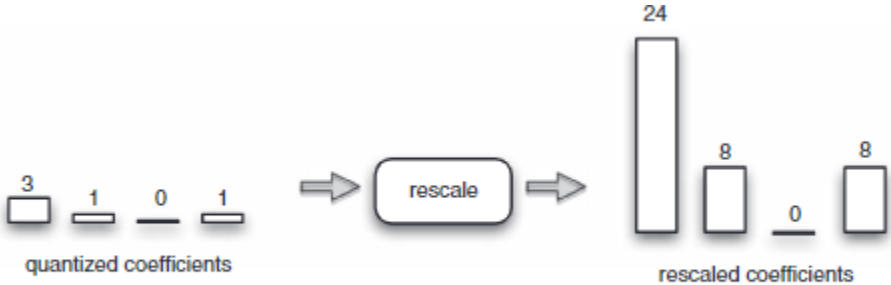
Figure 4.14 Rescaling example
