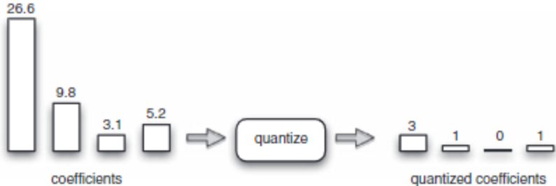
Figure 4.12 Quantization example
