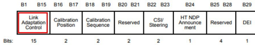
Figure 9-9—HT Control Middle subfield of the HT variant HT Control field
