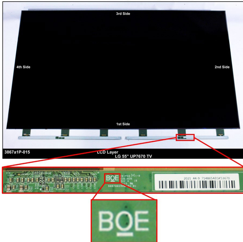
LG 55" UP7670PUC, LCD Layer (front)
