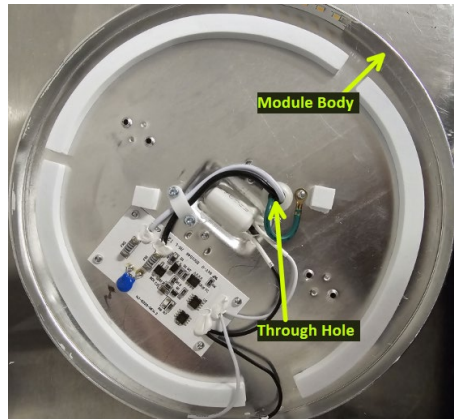
Figure 4B - 6 Traverse – Round 7” (3)
