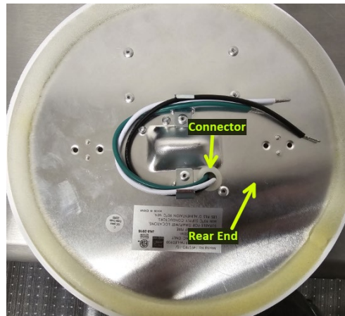
Figure 4B - 7 Traverse – Round 7” (1)
