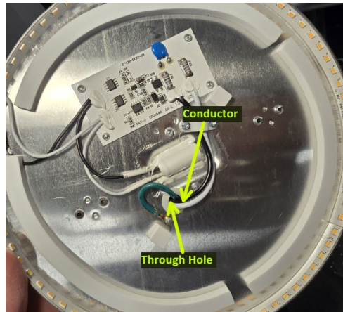
Figure 4B - 8 Traverse – Round 7” (2)
