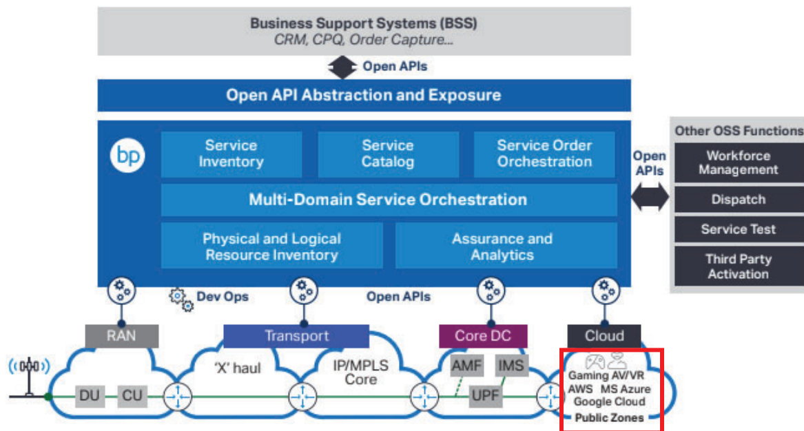
Figure 1. Blue Planet 5G Network Slicing solution architecture
